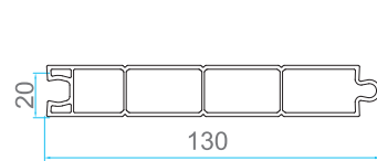
AP 510 PANEL PROFILE
