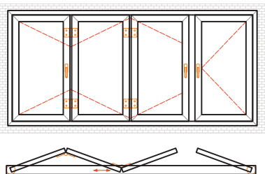
SLIDE & FOLD DOOR-431 OUTWARD OPENING
