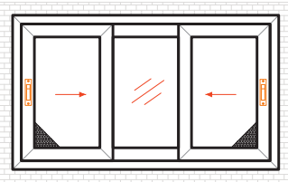
SLIDING WINDOW WITH MESH (2.5T 3P) CENTER FIXED
