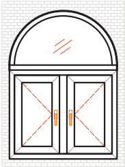
CASEMENT WINDOW-DOUBLE OPEN WITH TOP FIX-ARCH (OUTWARD OPENING)
