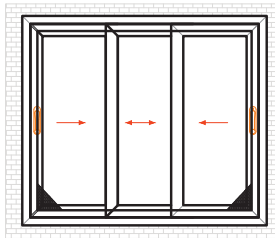
SLIDING WINDOW / DOOR (3T 3P) WITH MESH
