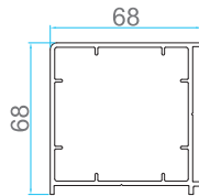
AP 501 SQ.BAY POLE (60X60)
