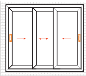
SLIDING WINDOW / DOOR (3T 3P)
