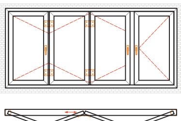
SLIDE & FOLD DOOR-431 INWARD OPENING
