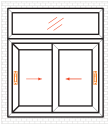
SLIDING WINDOW / DOOR (2T 2P)-Top Fix
